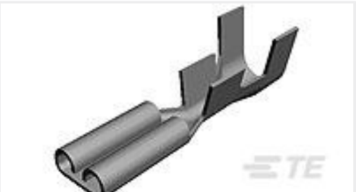
TE Part #42169-2 SPRING SPADE TERMINAL 18-14 AWG TPBR
