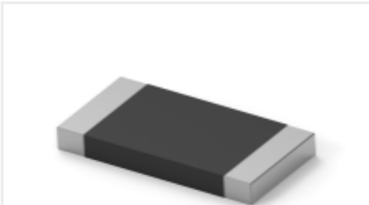
TE Part #3-2176421-7 TLRP 2512 2.0W R100 1% 25PPM 4K RL
