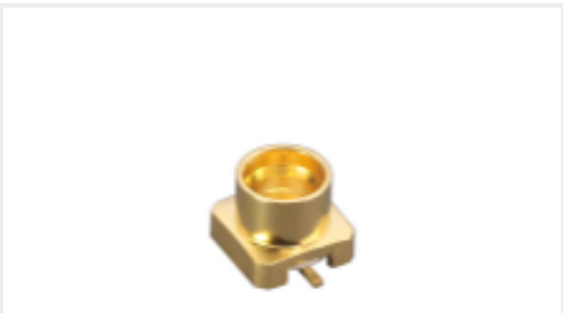
TE Part #CONSMP001-SMD-G-T SMP Plug 50 Ohm PCB Surface Mount
