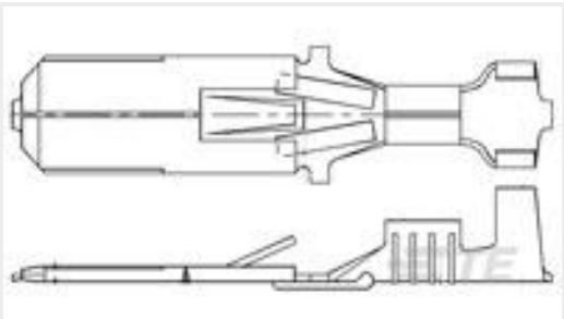
TE Part #160451-2 FF 250 TAB 18-14AWG TPPB LP
