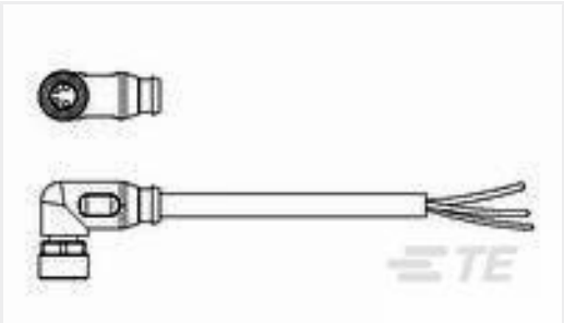
TE Part #1-2273011-3 M8 x 1.0 Angled socket Pigtail
