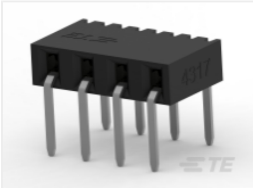
TE Part #2314938-4 4P,2MM,B-B,REC,SRHZ,2.8,0.76AU,TR
