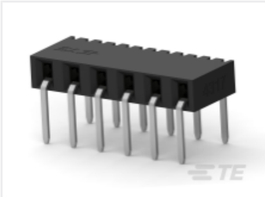
TE Part #2314938-6 6P,2MM,B-B,REC,SRHZ,2.8,0.76AU,TR
