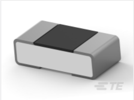
TE Part #3-2176364-7 RQ 0402 11K 0.1% 10PPM 5K RL
