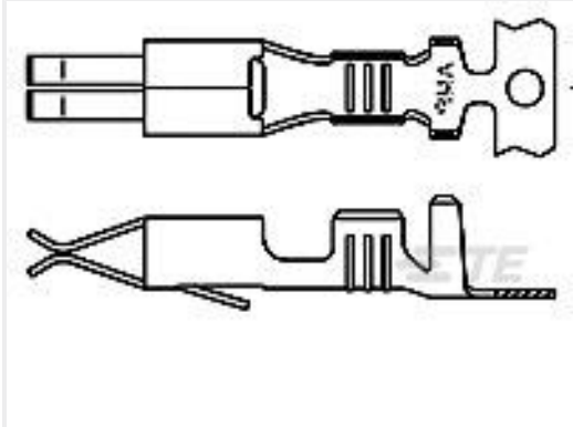
TE Part #643222-1 MINI-SPRING RECEPTACLE 20-16 AWG PTPBR
