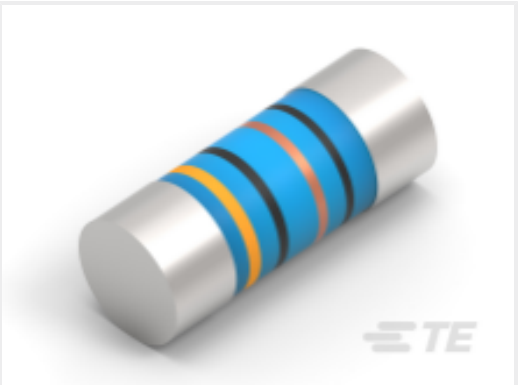
TE Part #9-2176316-4 MELF SMA-A 330K 1% 50PPM 0207 1W
