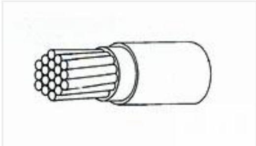
TE Part #267522-000 22759/34-14-0
