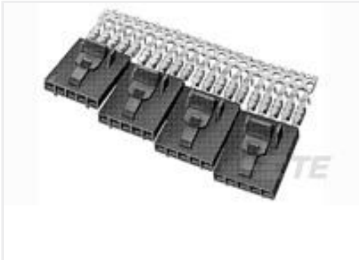
TE Part #5-103957-7 2X8 MTE RCPT SR LATCH .100CL
