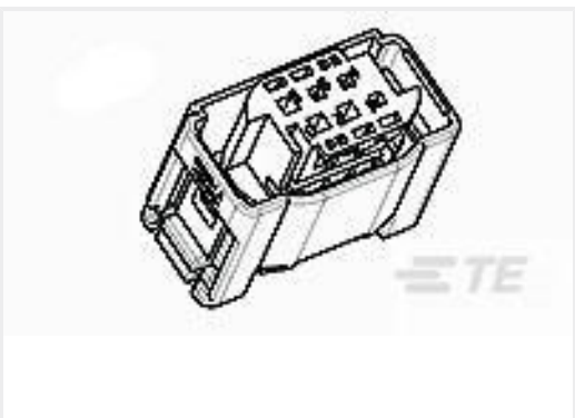
TE Part #2-967616-1 6POS MQS REC SEALED COD B
