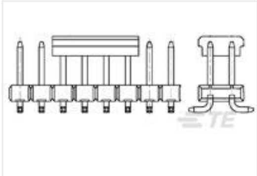
TE Part #966926-5 2X5P MODU 2MM PIN HDR,SMD, BLSTR
