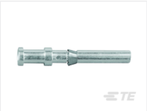
TE Part #T2020002005-000 CDF-0.5
