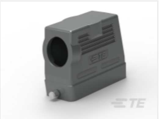
TE Part #T1330160140-000 H16B-TSH-RO-M40
