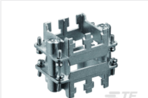
TE Part #T2070244201-000 H24BN-T6-F
