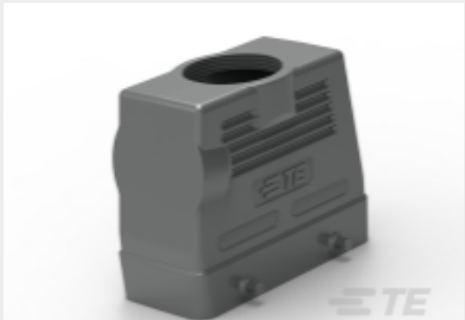
TE Part #T1240160140-000 H16B-TGH-M40
