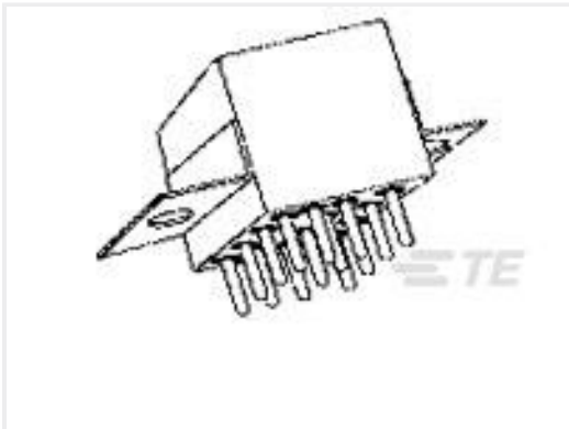
TE Part #8-1617760-6 FCB-405-0625M=M83536/6-025M
