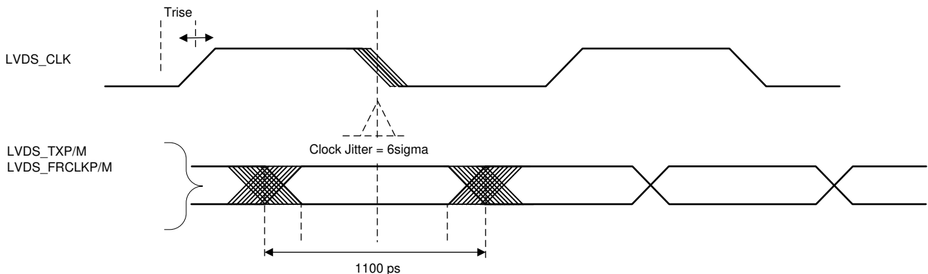
Figure 7-16. Timing Parameters
